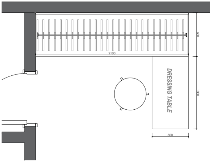
MASTER ROOM WARDROBE PLAN
